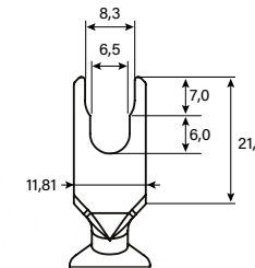
Multi-Spade Dimensions (mm)
