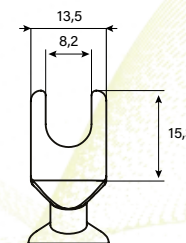
U-Spade Dimensions (mm)
