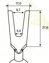
V-Spade Dimensions (mm)
